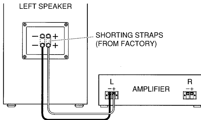
FIGURE 2 – Speaker connection
